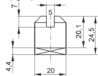
Coupling
