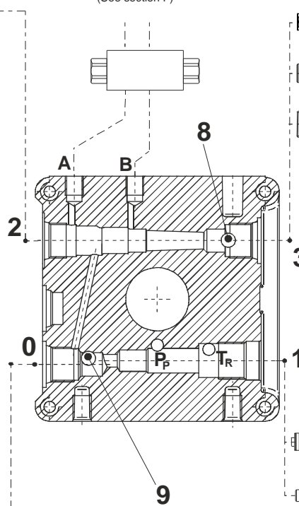
Modular manifold with check valves (See section F)
