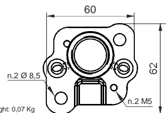
Aluminium adapter flange for group 0 Code: E60513025
