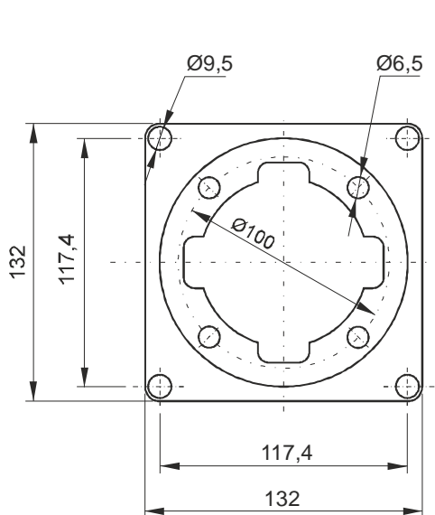
Adaptor flange
