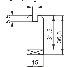
Pump group 0 side E36100006
