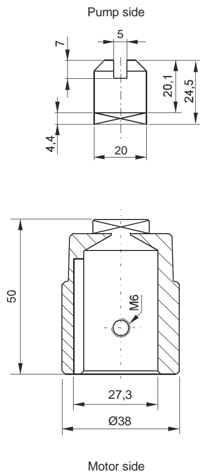
Coupling
